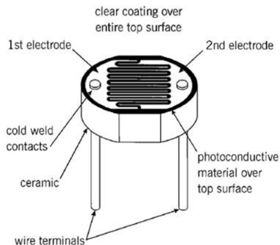
Fig 2.8 LDR Sensor
