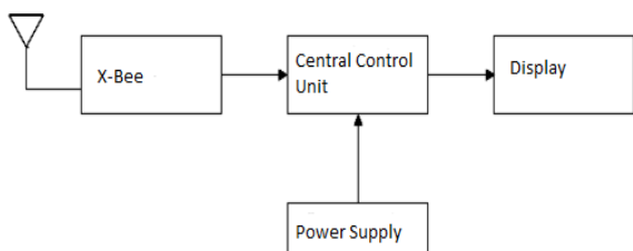
Figure 2.9: Base station
